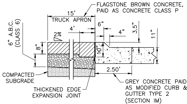
A-A Typical Truck Apron Detail
