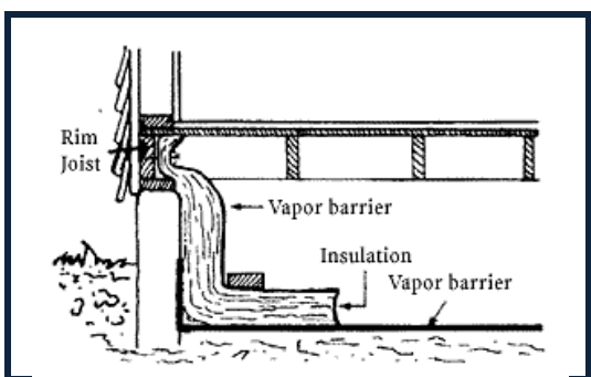
Conditioned Crawlspace
