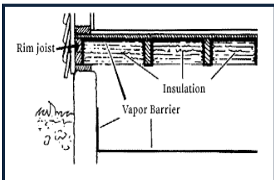
Unconditioned Crawlspace
