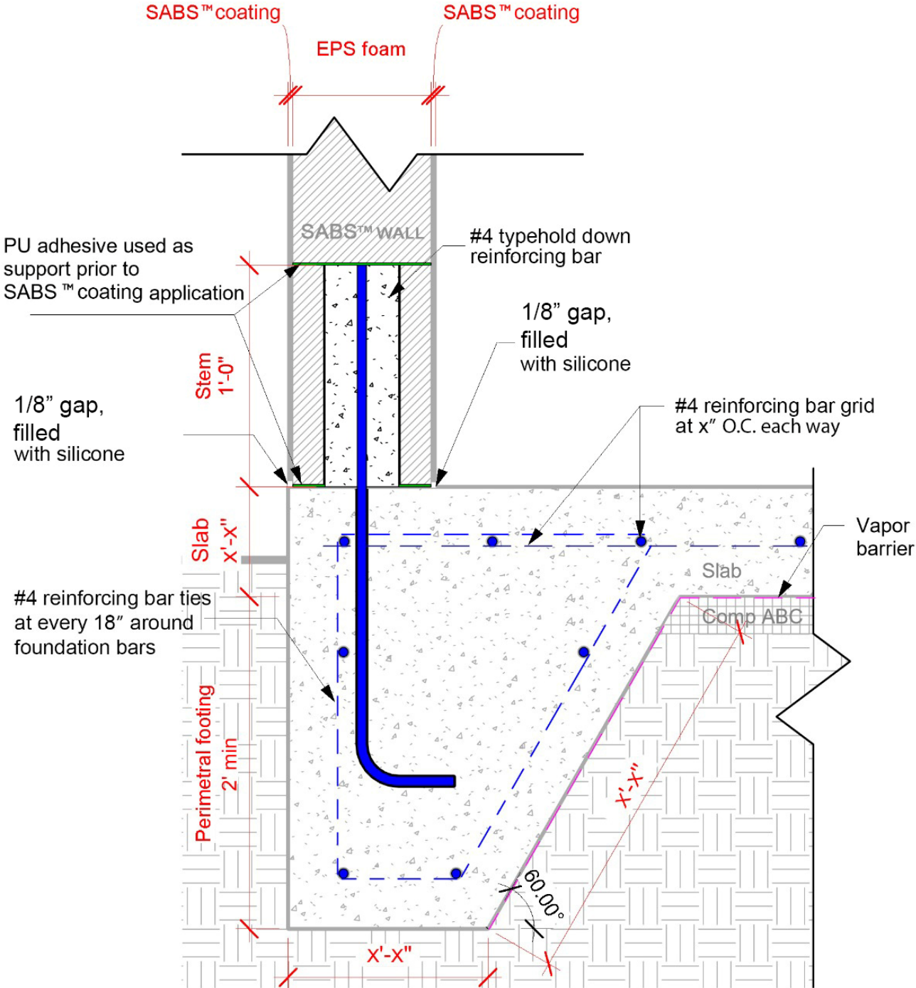
FIGURE 2—TYPICAL DETAILS (must be designed by registered design professional)
