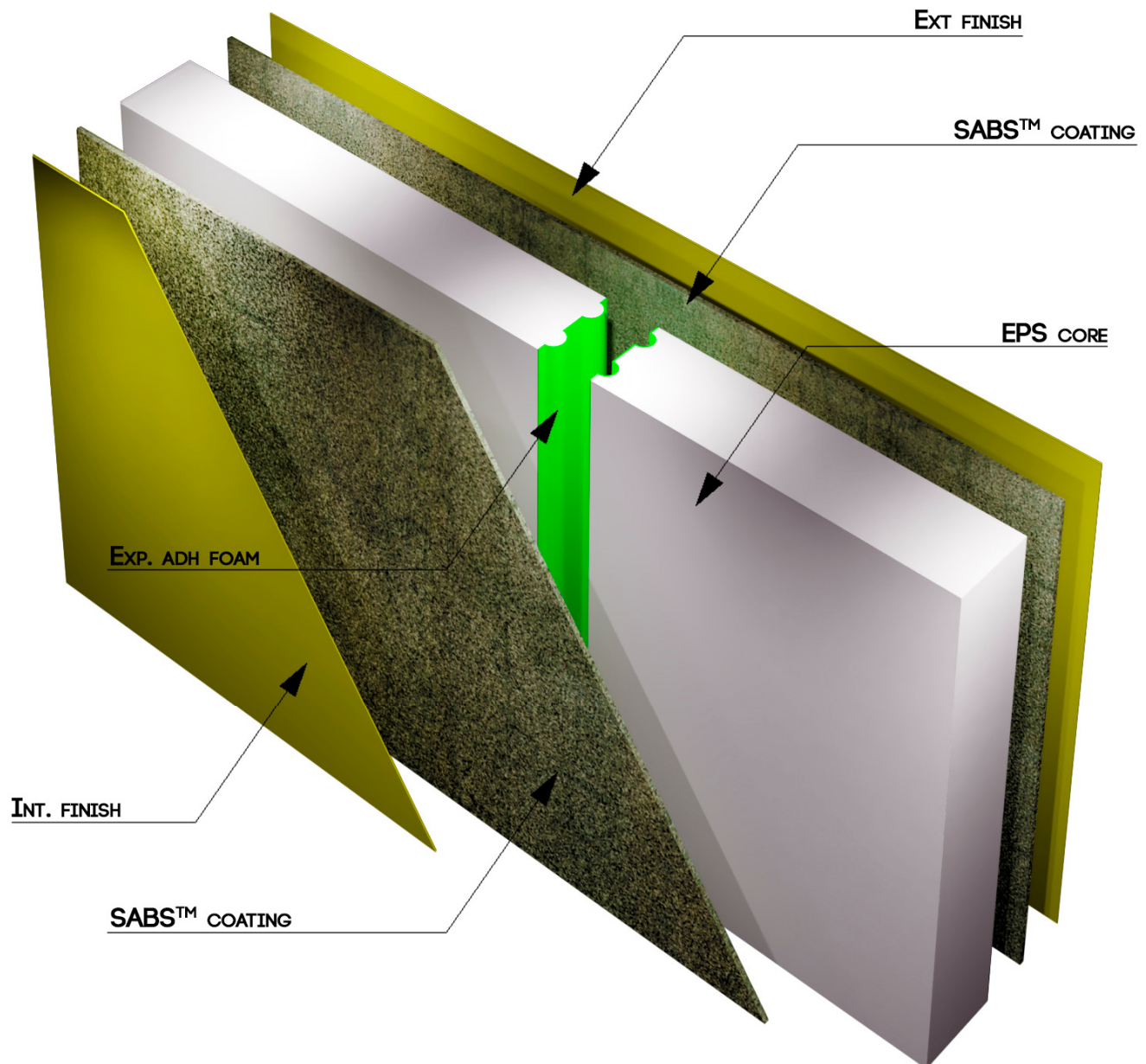
FIGURE 1—FLAT ELEMENTS
