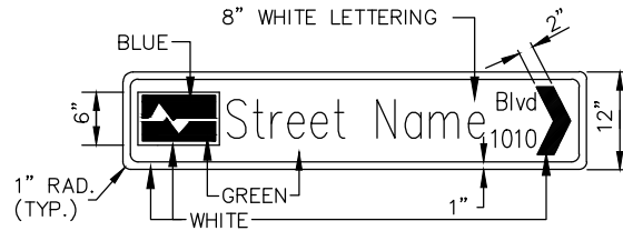
D1-1, Street Name Detail Sign
