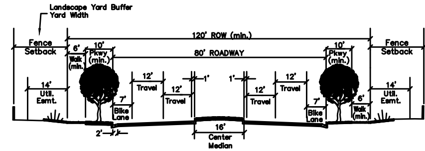
(4-LANE ARTERIAL)
