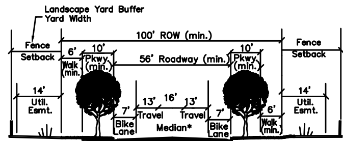
(2-LANE ARTERIAL)
