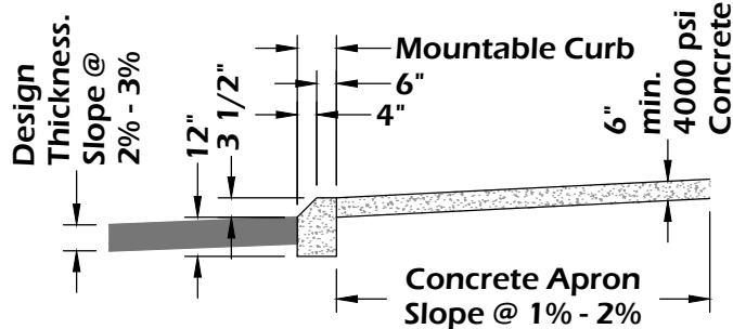
A-A Typical Truck Apron Detail
