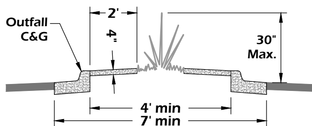
B-B Typical Splitter Island Detail
