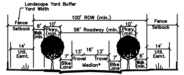
2-LANE ARTERIAL/2-LANE ARTERIAL
