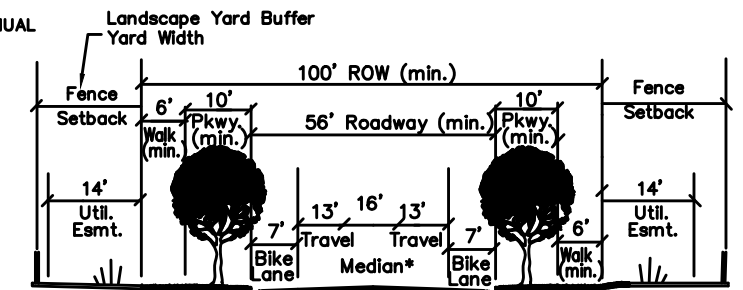
(2-LANE ARTERIAL)
