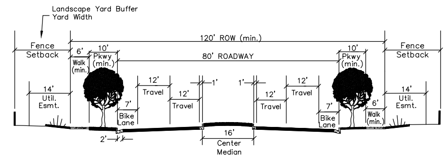
4-LANE ARTERIAL/4-LANE ARTERIAL
