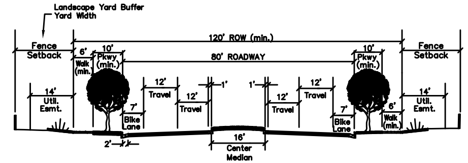
(4-LANE ARTERIAL)
