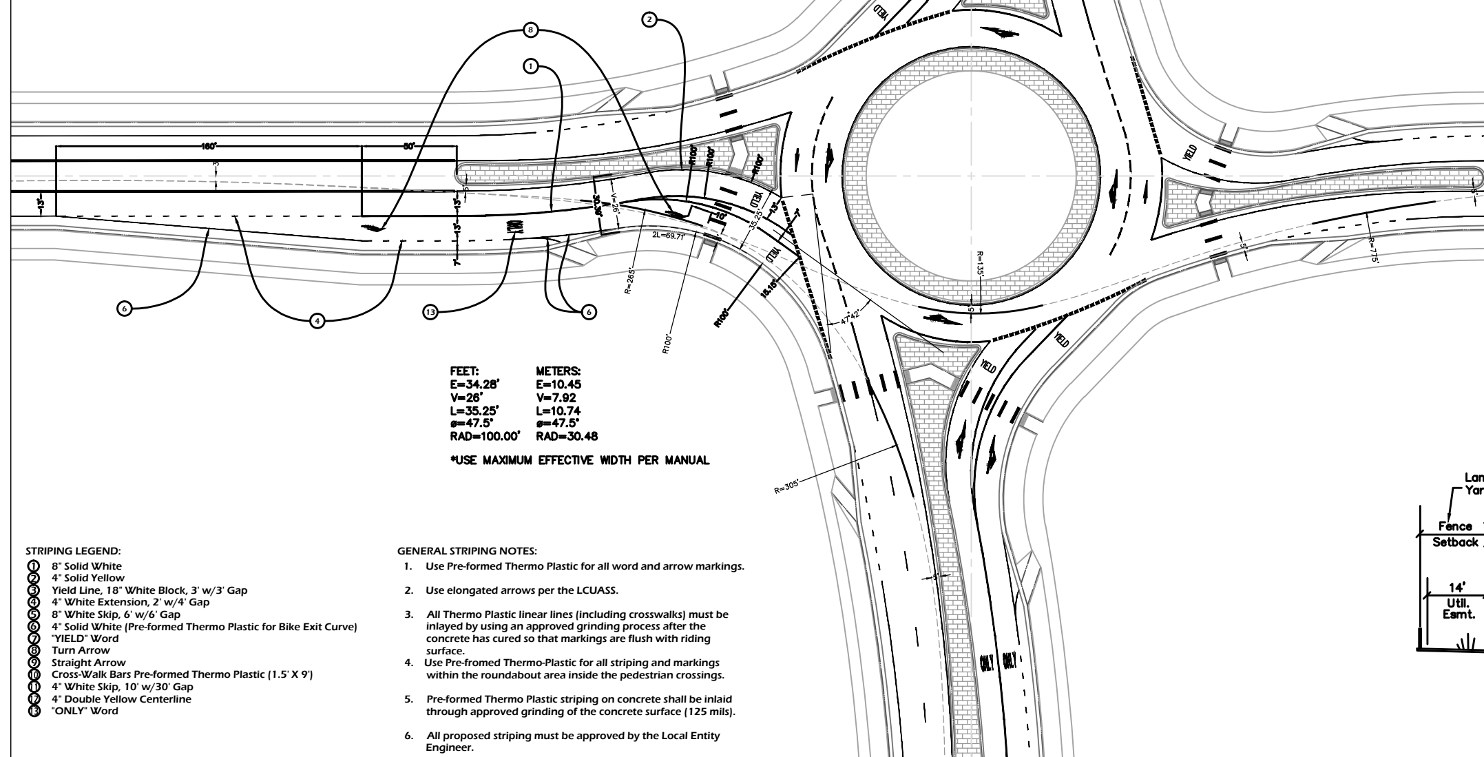
(2-LANE ARTERIAL)
