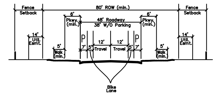
COLLECTOR/COLLECTOR
